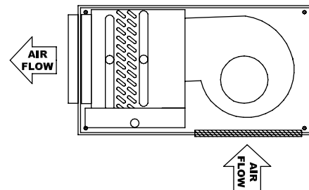
THHE DUCTED SUPPLY AND SINGLE DEFLECTION BOTTOM RETURN GRILLE
