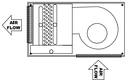
THHE DOUBLE DEFLECTION SUPPLY GRILLE AND SINGLE DEFLECTION BOTTOM RETURN GRILLE
