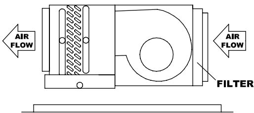
THHP REAR RETURN WITH SOLID ACCESS PANEL
