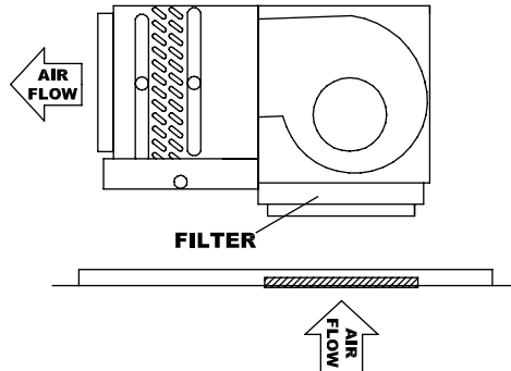
THHP BOTTOM RETURN W/BOTTOM CEILING PANEL
