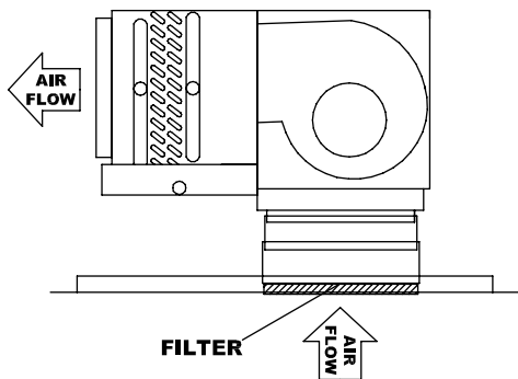
THHP BOTTOM RETURN WITH TELESCOPING BOTTOM PANEL
